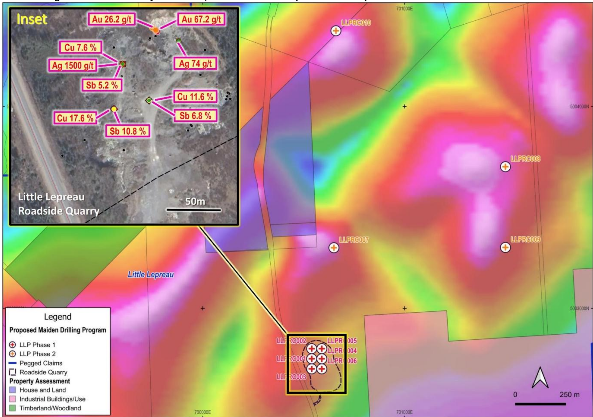
Figure 2: Little Lepreau Prospect, illustrating the proposed drillhole locations overlaid on government 440m magnetic dataset 3 .
