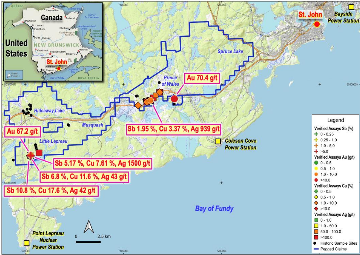
Figure 1: Saint John Project location, tenure and rock chip results overlaid on infrastructure and Cadastral data 2 .
